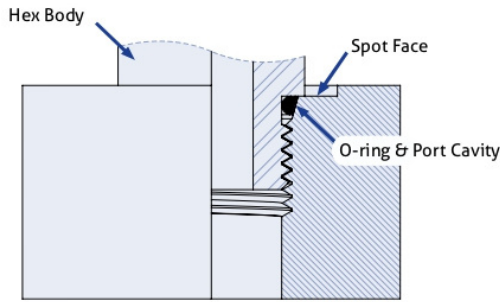
Figure 23: Straight ISO 6149
