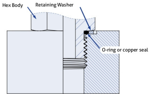
Figure 17: BSPP & Metric Straight (DIN 3852-1 & -2)
