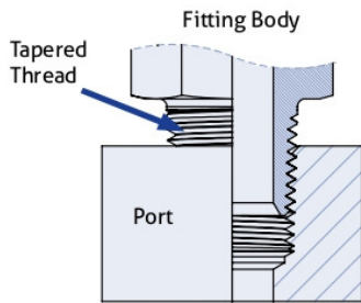
Figure 14: BSPT Assembly
