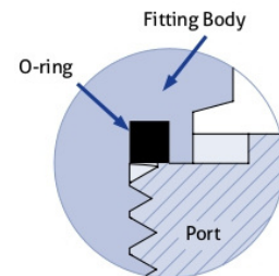
Figure 21: Elastomeric Seal
