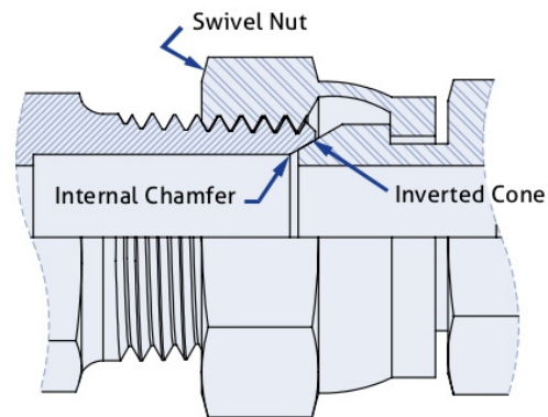
Figure 15: BSPP Union
