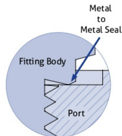
Figure 20: Cutting Face Seal
