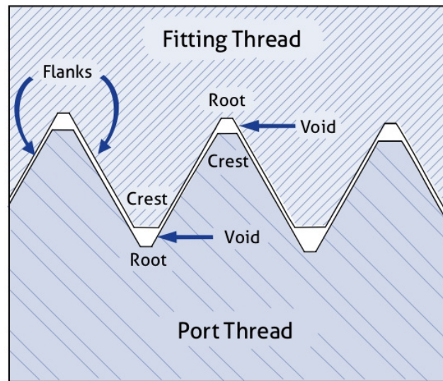
Figure 3 : NPT Thread View
