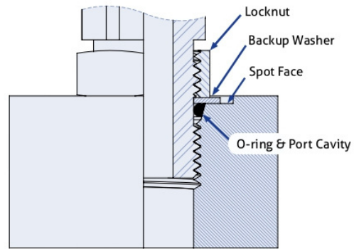
Figure 24: Adjustable ISO 6149
