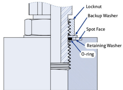
Figure 18: BSPP & Metric Adjustable (DIN 3852-1 & -2)
