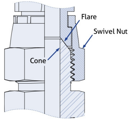
Figure 4: Flare Fitting Assembly
