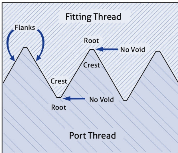
Figure 2 : NPTF Thread View
