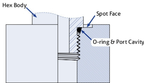
Figure 5 : Straight SAE ORB
