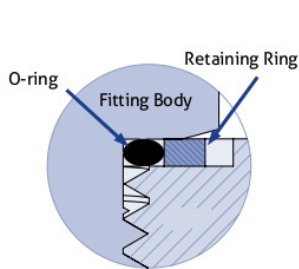
Figure 19: Retaining Ring with O-ring Seal
