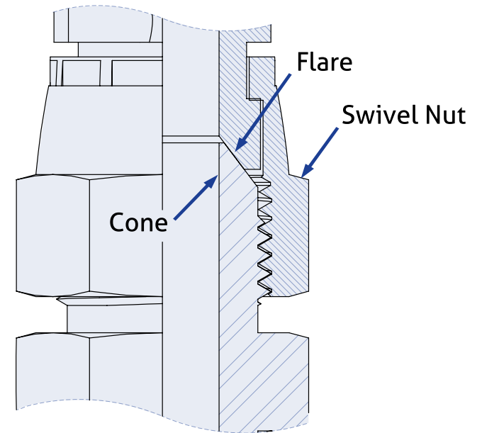
Figure 4: Flare Fitting Assembly
